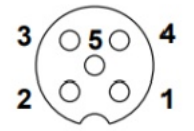
M 12 female connector
